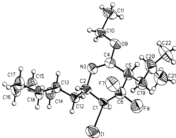
Figure 1. Molecular structure and labeling scheme for ( \pm )- 8 (50% thermal ellipsoids).
