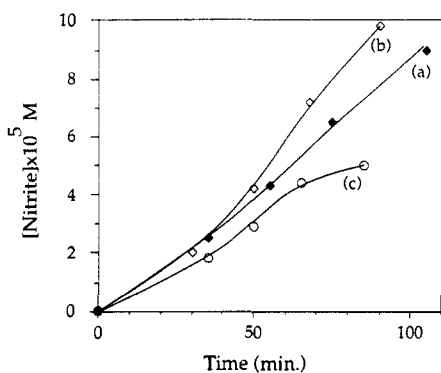
Figure 1. Rate of \text{NO}_3^- reduction in the assembly composed of nitrate reductase (0.023 unit, based on native enzyme) immobilized in the acrylamide (1) copolymer. In all experiments, [\text{NO}_3^-] = 4.4 \times 10^{-3} \text{ M} in 2.3 mL of Tris buffer, \text{pH} = 7.44 . (a) Dark reduction in the presence of sodium dithionite, 9.4 \times 10^{-3} \text{ M} . (b) Through illumination in the presence of \text{Ru}(\text{bpy})_3^{2+} ( 5.5 \times 10^{-5} \text{ M} ) and \text{Na}_2\text{EDTA} ( 4.4 \times 10^{-3} \text{ M} ). (c) Through illumination in the presence of \text{Ru}(\text{bpy})_3^{2+} ( 5.5 \times 10^{-5} \text{ M} ), \text{Na}_2\text{EDTA} ( 4.4 \times 10^{-3} \text{ M} ), and added \text{MV}^{2+} ( 3.3 \times 10^{-4} \text{ M} ), where the enzyme is immobilized in a nonfunctionalized acrylamide polymer.
